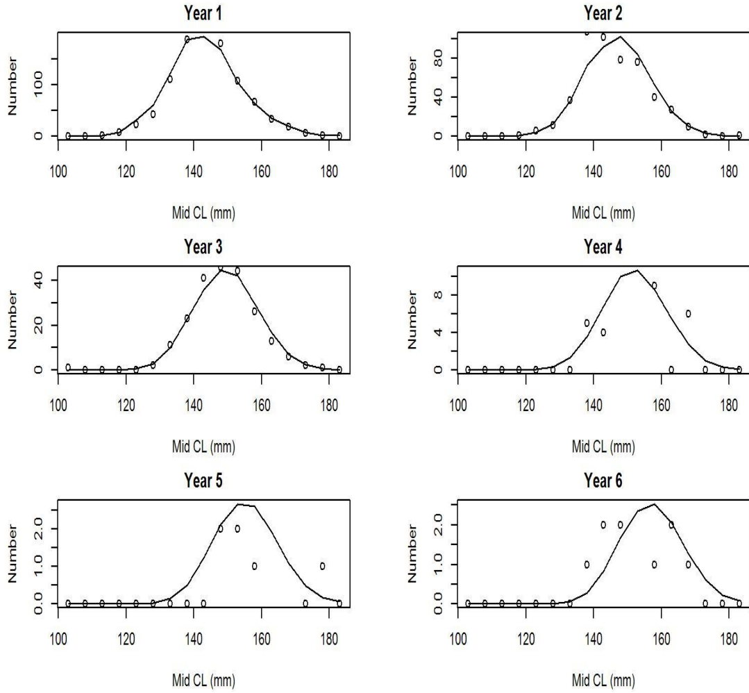
Figure 15. Observed (open circles) vs. predicted (solid line) tag recaptures by size bin for years 1 to 6 recaptures under scenario 17_0 for EAG golden king crab.
