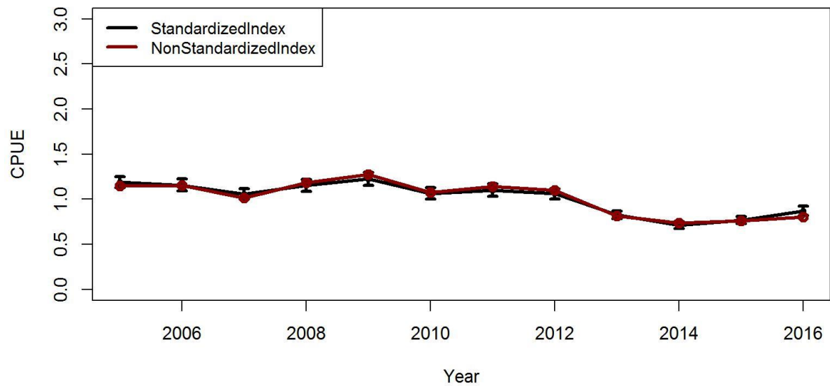
Figure B.3. Trends in non-standardized [arithmetic (nominal)] and standardized (negative binomial GLM) CPUE indices with \pm 2 SE for Aleutian Islands golden king crab observer data from WAG (east of 174^\circ W longitude). Top panel: 1995/96–2004/05, and bottom panel: 2005/06–2016/17. Standardized indices: black line and non-standardized indices: red line. Variable selection by R^2 criteria.
