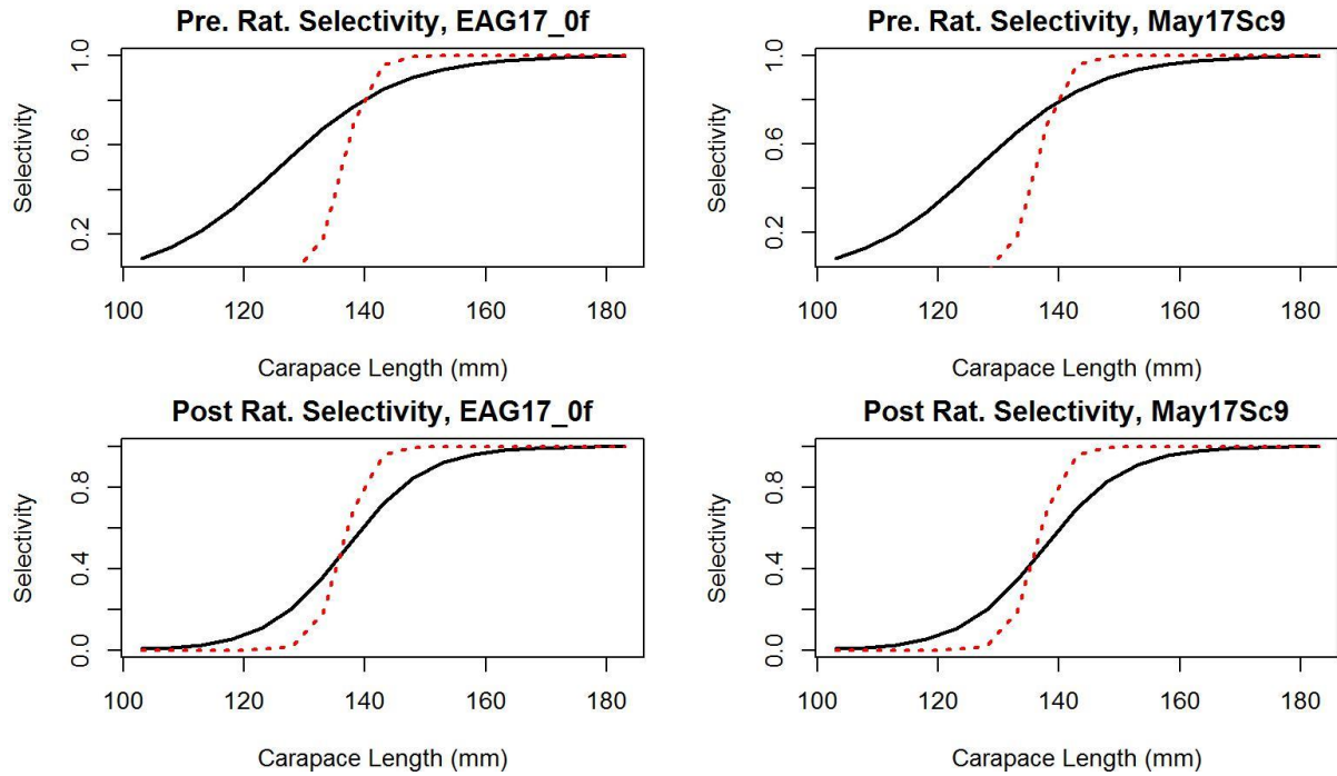
Figure 14. Estimated total (black solid line) and retained selectivity (red dotted line) for pre- and post-rationalization periods under scenarios 17_0 to May 2017 Sc9 model fits to golden king crab data in the EAG .
