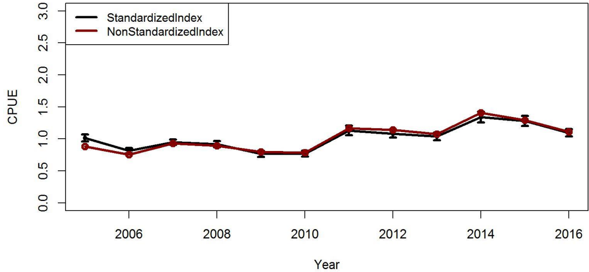
Figure B.1. Trends in non-standardized [arithmetic (nominal)] and standardized (negative binomial GLM) CPUE indices with \pm 2 SE for Aleutian Islands golden king crab observer data from EAG (east of 174^\circ W longitude). Top panel: 1995/96–2004/05, and bottom panel: 2005/06–2016/17. Standardized indices: black line and non-standardized indices: red line. Variable selection by R^2 criteria.
