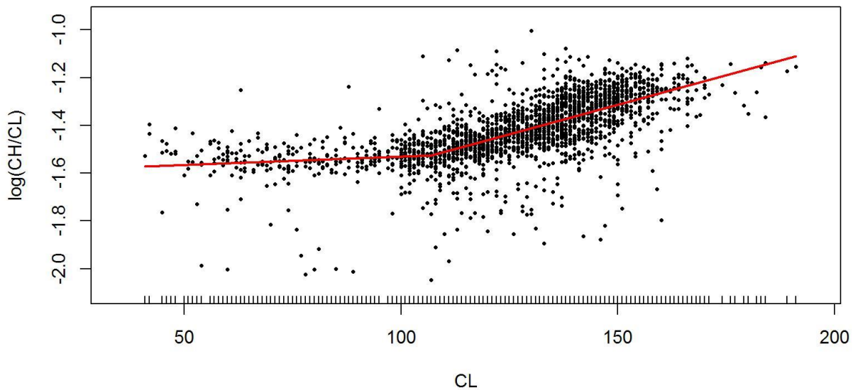
Figure C.1. Segmented linear regression fit to ln(CH/CL) vs. CL data of male golden king crab in EAG .
