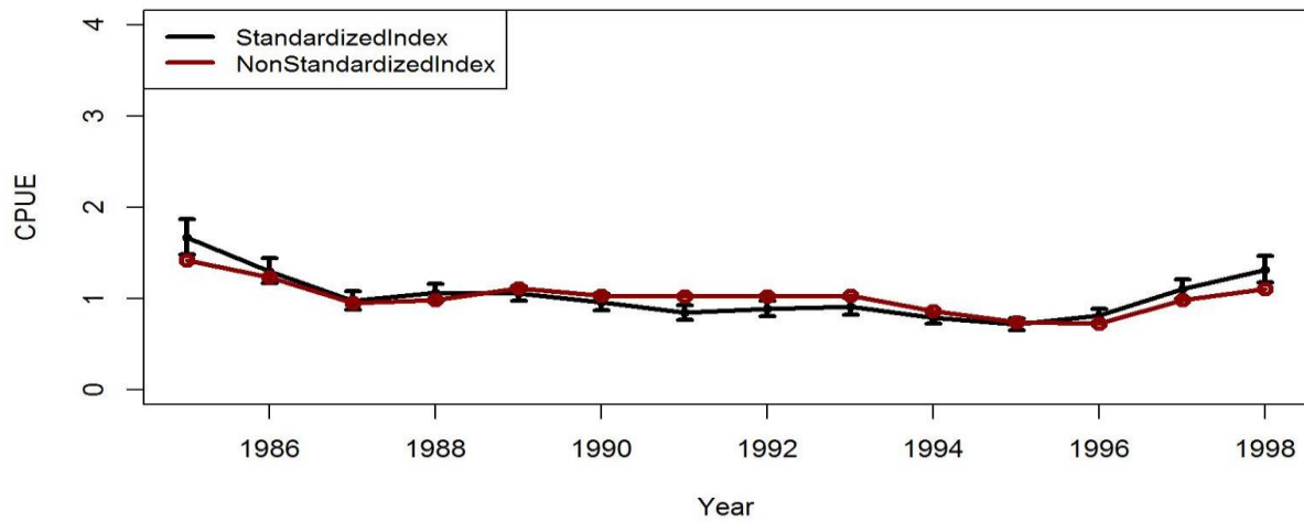
Figure B.8. Trends in non-standardized [arithmetic (nominal)] and standardized (lognormal GLM) CPUE indices with +/- 2 SE for Aleutian Islands golden king crab from EAG . The 1985/86–1998/99 fish ticket data set was used. Standardized indices: black line and non-standardized indices: red line. Top panel: variable selection by R 2 criteria; bottom panel: variable selection by AIC criteria.
