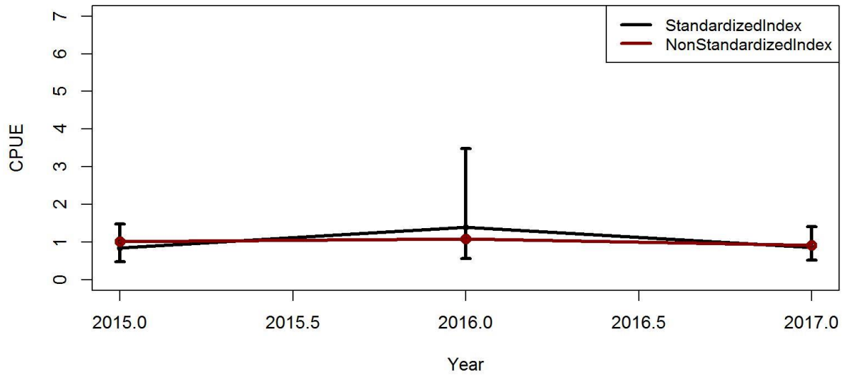
Figure B.5. Trends in non-standardized [arithmetic (nominal)] and standardized (negative binomial GLM) CPUE indices with \pm 2 SE for Aleutian Islands golden king crab independent survey data from EAG (east of 174 ° W longitude) during 2015–2017. Standardized indices: black line and non-standardized indices: red line. Variable selection by R^2 criteria.
