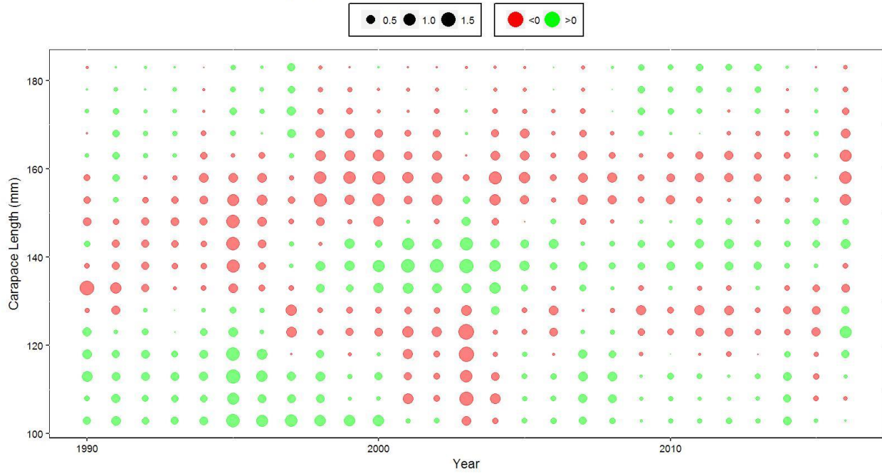
WAG 17_0d Total Catch Size Composition Standardized Residuals
