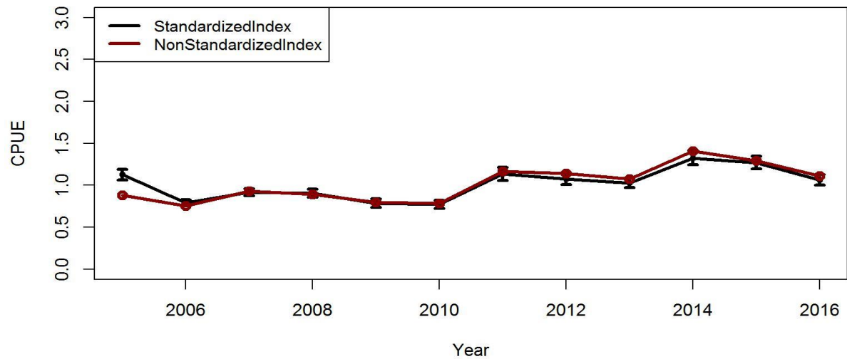
Figure B.2. Trends in non-standardized [arithmetic (nominal)] and standardized (negative binomial GLM) CPUE indices with \pm 2 SE for Aleutian Islands golden king crab observer data from EAG (east of 174 ° W longitude). Top panel: 1995/96–2004/05, and bottom panel: 2005/06–2016/17. Standardized indices: black line and non-standardized indices: red line. Variable selection by AIC criteria.
