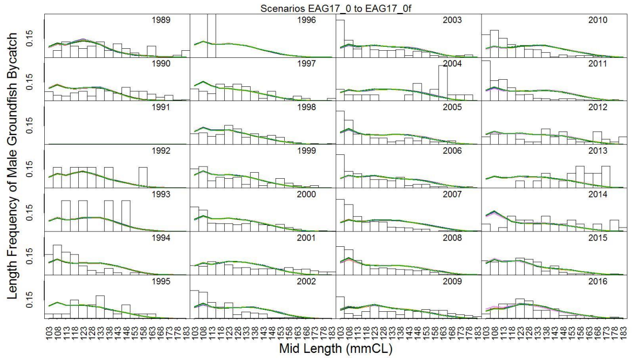
Figure 13. Predicted (line) vs. observed (bar) groundfish (or trawl) discarded bycatch relative length frequency distributions under scenarios 17_0 to 17_0f for golden king crab in the EAG , 1989/90 to 2016/17. Note that this data set was not used in the model fitting.
