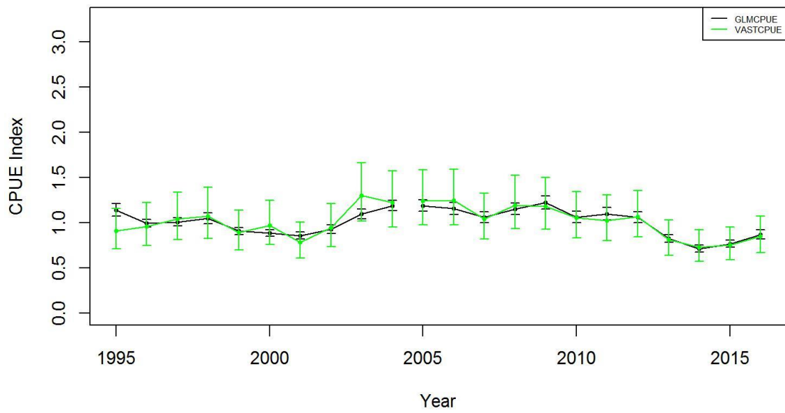
Figure B.7. Comparison of GLM (black) and VAST (green) estimated CPUE indices with +/- 2 SE for Aleutian Islands golden king crab in EAG (top panel) and WAG (bottom panel) for 1995/96–2016/17. GLM variable selection by R^2 criteria.
